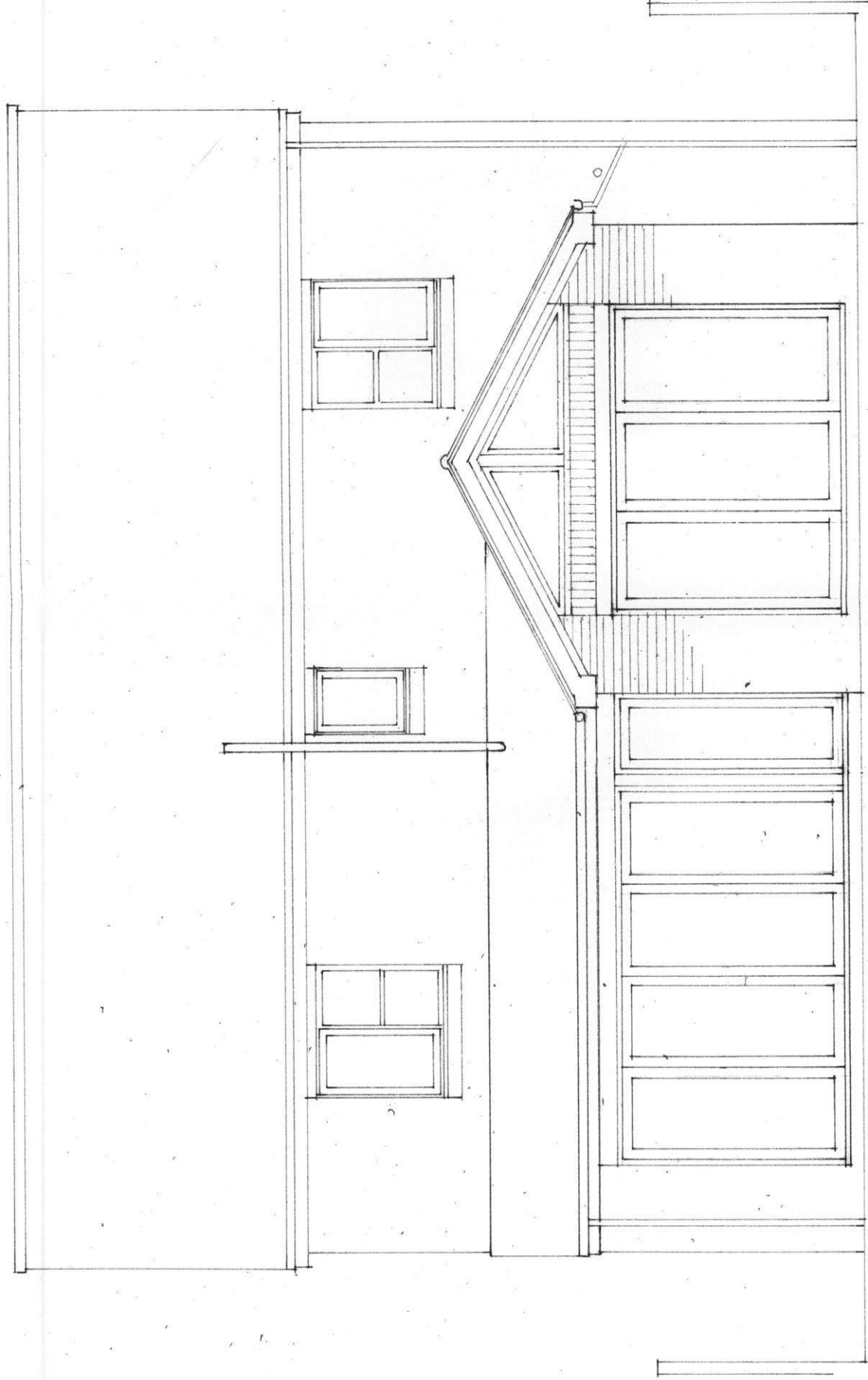
EAST ELEVATION
